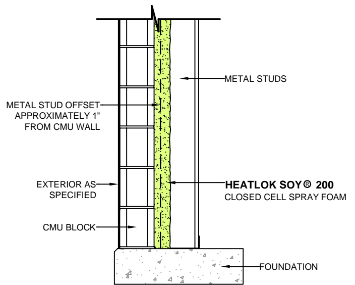
2 WALL DETAIL TYP. CMU BLOCK HEATLOK SOY IN METAL STUD CAVITY SECTION VIEW SCALE: 1-1/2" = 1'-0"
