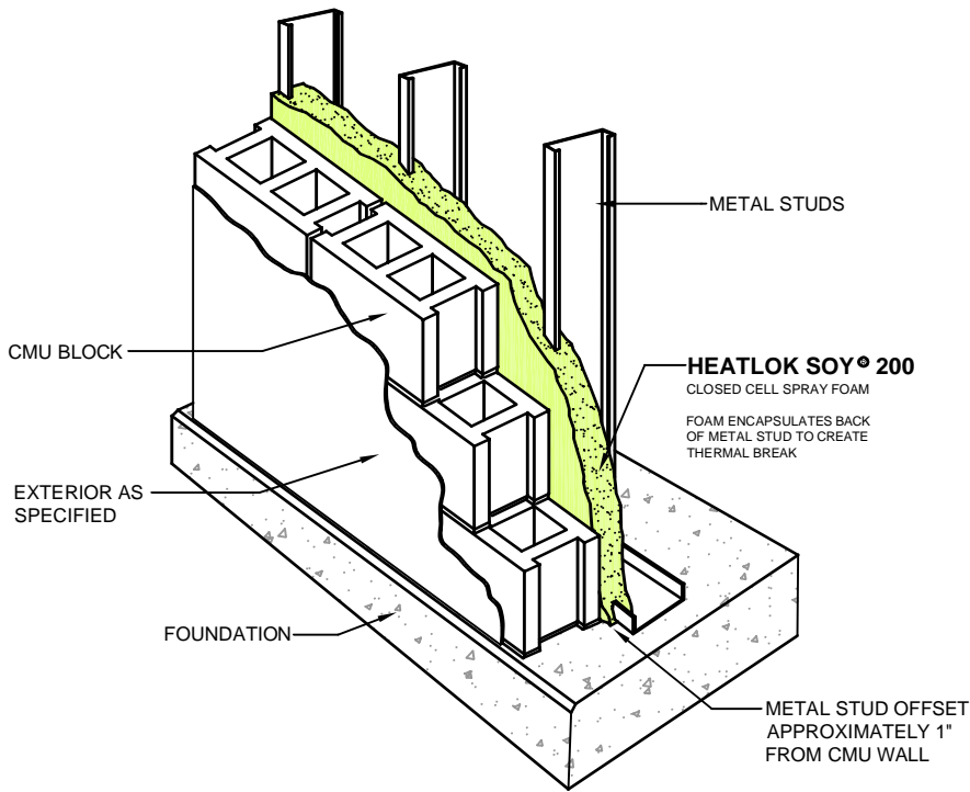
1 WALL DETAIL TYP. CMU BLOCK HEATLOK SOY IN METAL STUD CAVITY ISOMETRIC VIEW SCALE: 1" = 1'-0"
